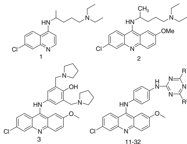
Figure 1. Structure of CQ, quinacrine, pyronaridine and title compounds.
