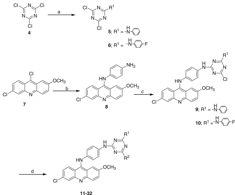
Scheme 1. Reagents and conditions: (a) aniline/ p -fluoroaniline, THF, 0 °C temp, 2 h; (b) p -phenylenediamine, p -TSA, absolute ethanol, reflux, 3 h; (c) monosubstituted triazines, dry THF, reflux, 10 h; (d) various amines, dry THF, 65 °C, 4 h.
